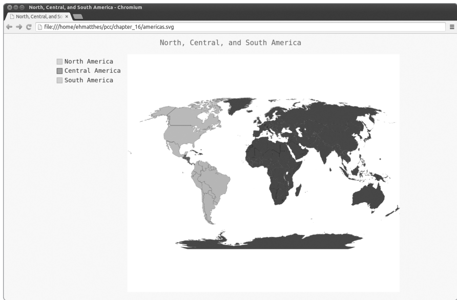
Figure 16-7: A simple instance of the Worldmap chart type
